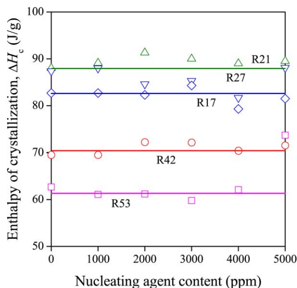
Figure 2. Enthalpy of crystallization plotted against the concentration of the sorbitol nucleating agent for polymers with various ethylene contents. Symbols: (□) R53, (○) R42, (▽) R27, (△) R21, (◇) R17. [Color figure can be viewed in the online issue, which is available at wileyonlinelibrary.com .]
