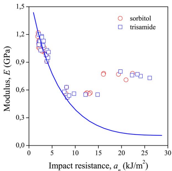
Figure 5. Stiffness of nucleated random copolymers plotted against their impact resistance. Symbols: (○) sorbitol, (□) trisamide. [Color figure can be viewed in the online issue, which is available at wileyonlinelibrary.com .]
