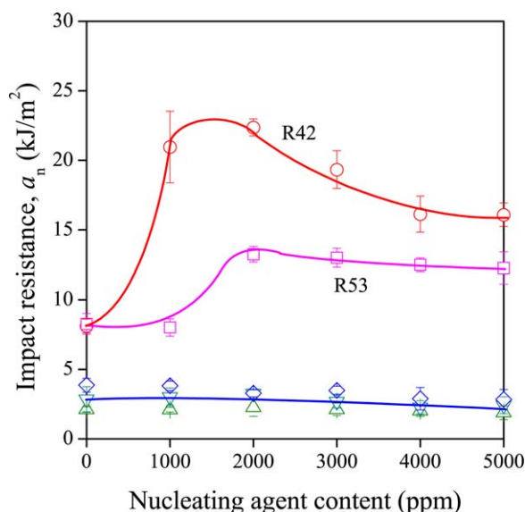
Figure 4. Effect of nucleation on the impact resistance of PP random copolymers. Nucleating agent: sorbitol. Symbols: (□) R53, (○) R42, (▽) R27, (△) R21, (◇) R17. [Color figure can be viewed in the online issue, which is available at wileyonlinelibrary.com .]
