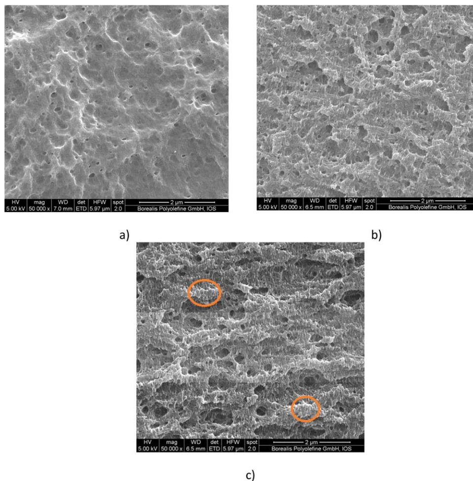
Figure 13. SEM micrographs taken from the etched cryo-cut surface of selected PP specimens. The slices were cut from the core of injection molded specimens parallel to flow direction. (a) neat R42 polymer, without nucleating agent, (b) R42, 2000 ppm sorbitol, and (c) R42, 4000 ppm sorbitol. [Color figure can be viewed in the online issue, which is available at wileyonlinelibrary.com .]
