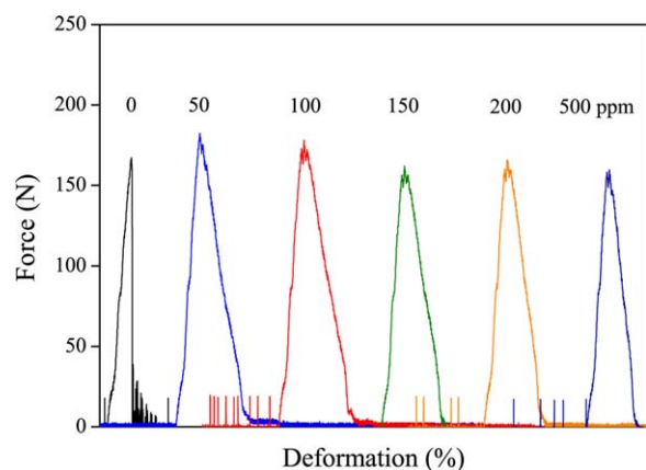
Figure 9. Effect of nucleation on the fracture of notched specimens prepared from the R42 PP copolymer. Nucleating agent: trisamide. [Color figure can be viewed in the online issue, which is available at wileyonlinelibrary.com.]
