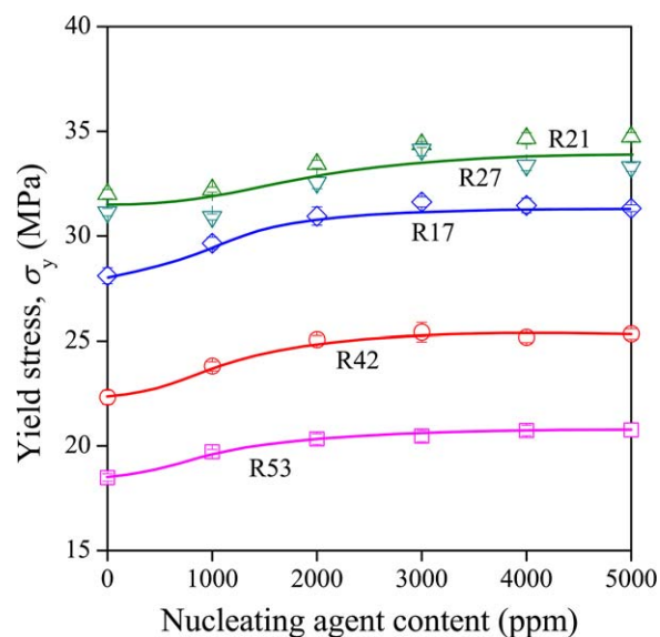
Figure 3. Dependence of the tensile yield stress of PP random copolymers on the amount of sorbitol nucleating agent added. Symbols: (□) R53, (○) R42, (▽) R27, (△) R21, (◇) R17. [Color figure can be viewed in the online issue, which is available at wileyonlinelibrary.com .]
