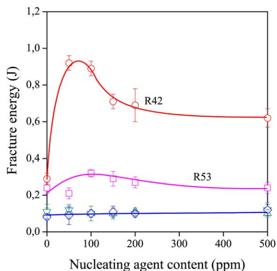
Figure 11. Fracture energy determined by instrumented impact testing plotted against the nucleating agent content of PP random copolymers containing the trisamide compound. Symbols: ( \square ) R53, ( \circ ) R42, ( \nabla ) R27, ( \triangle ) R21, ( \diamond ) R17. Nucleation: trisamide. [Color figure can be viewed in the online issue, which is available at wileyonlinelibrary.com.]
