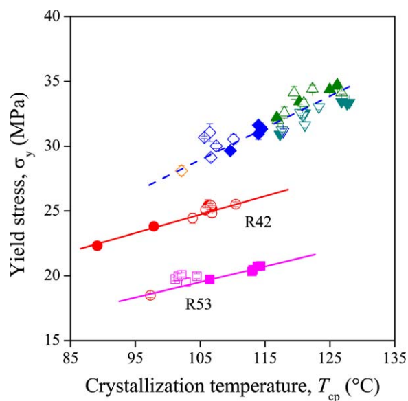
Figure 6. Correlation between the tensile yield stress and crystallization temperature (lamella thickness) of nucleated PP copolymers. Symbols: (□) R53, (○) R42, (▽) R27, (△) R21, (◇) R17. Full: sorbitol; empty: trisamide. [Color figure can be viewed in the online issue, which is available at wileyonlinelibrary.com.]
