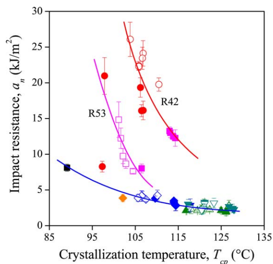
Figure 8. Correlation between the impact resistance and crystallization temperature of nucleated PP random copolymers. Symbols: (□) R53, (○) R42, (▽) R27, (△) R21, (◇) R17. Full: sorbitol; empty: trisamide. [Color figure can be viewed in the online issue, which is available at wileyonlinelibrary.com.]
