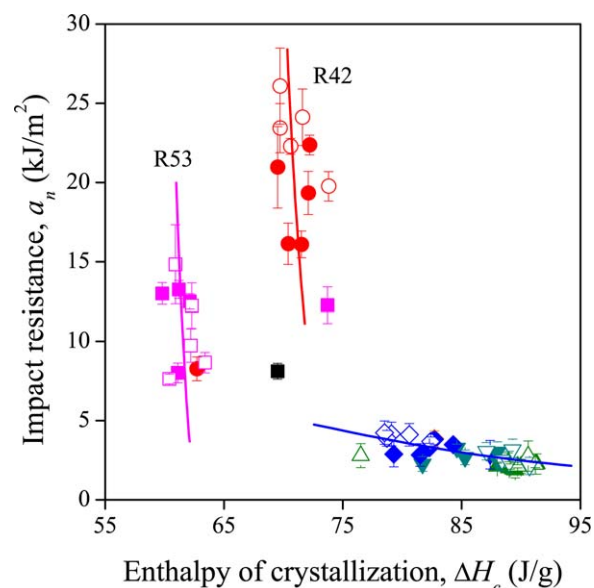
Figure 7. Lack of correlation between the impact resistance of nucleated random copolymers and their crystallinity (enthalpy of crystallization). Symbols: (□) R53, (○) R42, (▽) R27, (△) R21, (◇) R17. Full: sorbitol; empty: trisamide. [Color figure can be viewed in the online issue, which is available at wileyonlinelibrary.com.]
