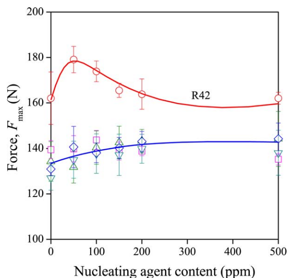
Figure 10. Effect of nucleation on crack initiation ( F_{\max} ) during the fracture of notched specimens prepared from nucleated PP copolymers. Symbols: ( \square ) R53, ( \circ ) R42, ( \nabla ) R27, ( \triangle ) R21, ( \diamond ) R17. Nucleation: trisamide. [Color figure can be viewed in the online issue, which is available at wileyonlinelibrary.com.]
