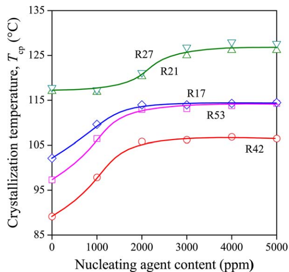
Figure 1. Effect of the molecular structure of the polymer and nucleation on the peak temperature of crystallization of PP random copolymers containing the sorbitol clarifier. Symbols: ( \square ) R53, ( \circ ) R42, ( \nabla ) R27, ( \triangle ) R21, ( \diamond ) R17. [Color figure can be viewed in the online issue, which is available at wileyonlinelibrary.com .]
