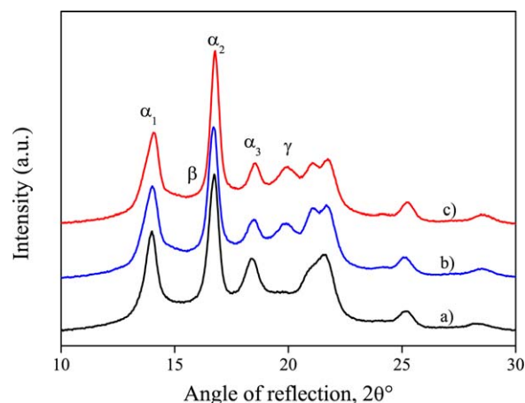
Figure 12. Effect of nucleation on the local morphology. Increase in the amount of the \gamma modification of PP upon nucleation. R42 copolymers; (a) neat, (b) 2000 ppm, (c) 4000 ppm sorbitol nucleating agent. [Color figure can be viewed in the online issue, which is available at wileyonlinelibrary.com.]
